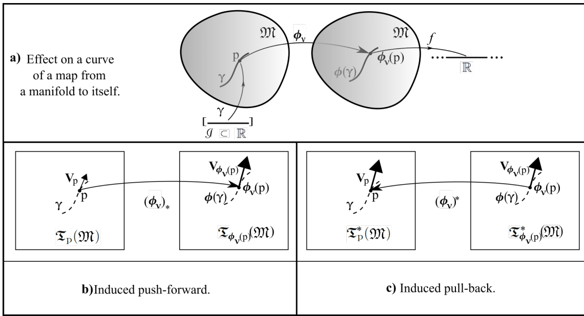
Figure 6: Curve, push and pull.
