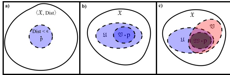
Figure 12: a) Infinitesimal neighbourhood in a metric space.
