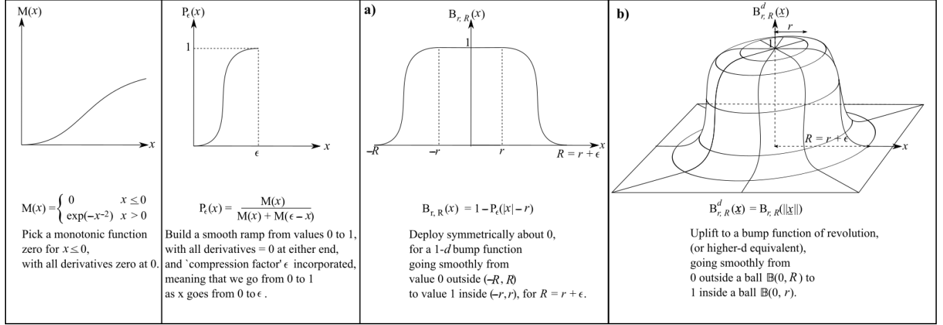
Figure 4: Bump functions on a) the interval (-R, R) in 1-d, and b) the open ball B^d(0, R) , using the same function as a radial profile for a surface of revolution bump function.
