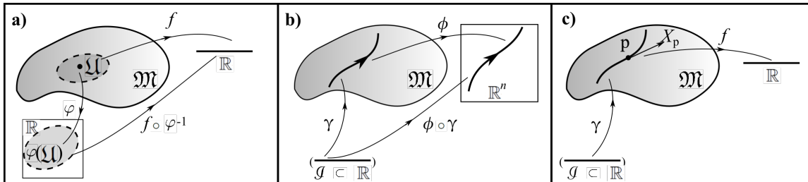
Figure 5: a) A function on a manifold.
