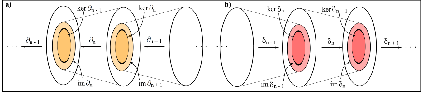
Figure 10: Spaces, maps, images and kernels in a) homology and b) cohomology.
