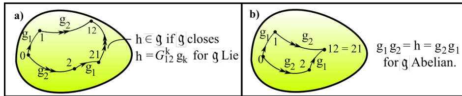
Figure 9: a) An algebra's commutator. This compares applying two transformations g_1, g_2 in either order to a common initial object 0. b) The even more straightforward commuting subcase, for which the final objects 12 and 21 coincide as well. Many instances of a) and b) occur in ALRoPoT, as picked out among the Series's figures by being depicted on lime-green egg-shaped spaces.
