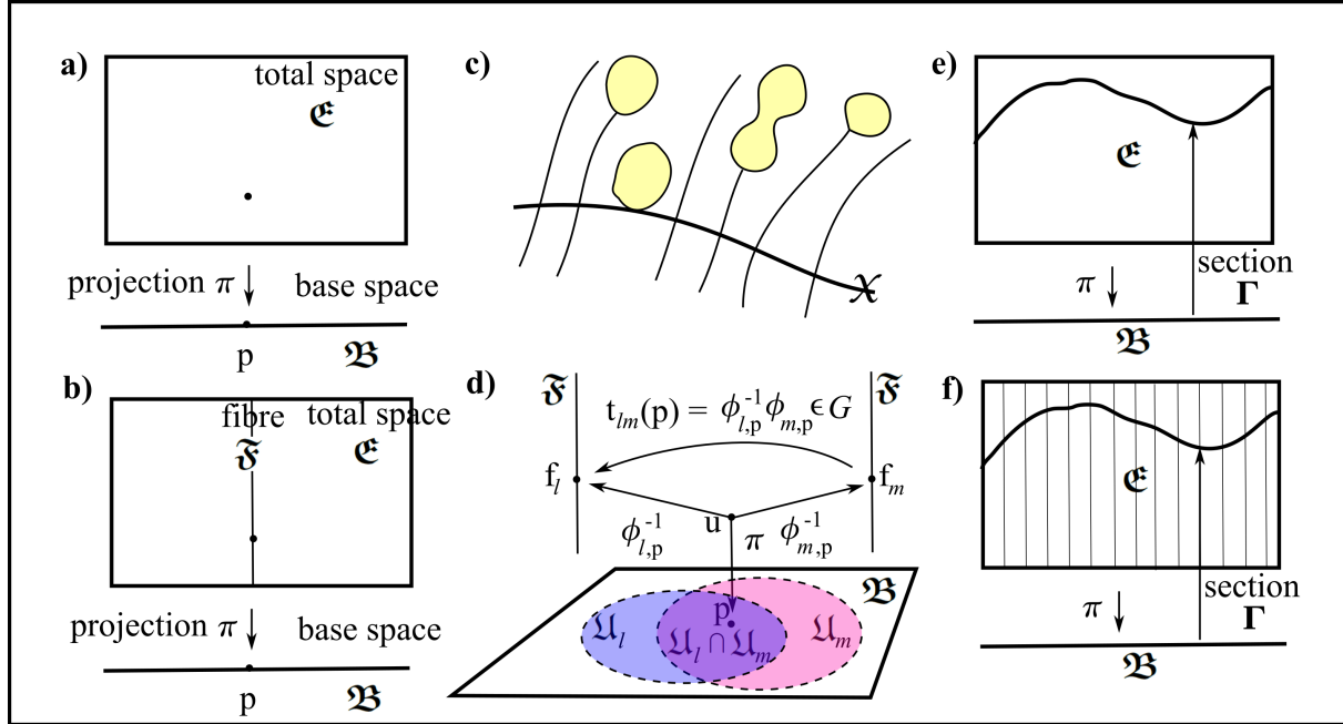
Figure 11: a) General bundle at the topological level.
