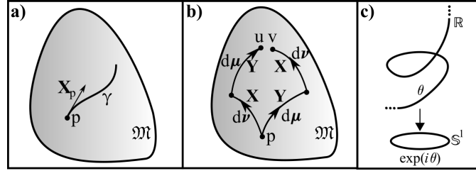
b) Commutator corresponding to proceeding along two local congruences of integral curves in either order.
